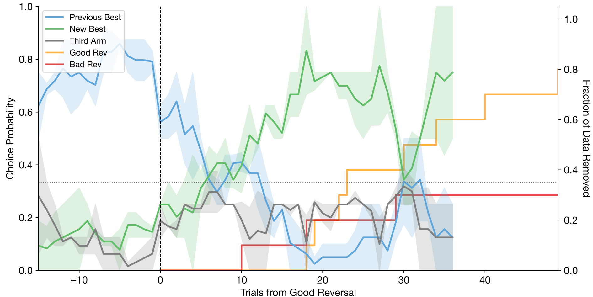
Good Reversal-Aligned Choices (mean \pm se across subjects | n=2 subjects, n=10 reversals)
